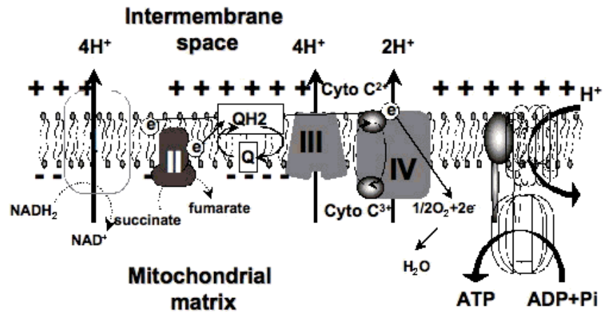
Figure 3. Structure of the mitochondrial respiratory chain
