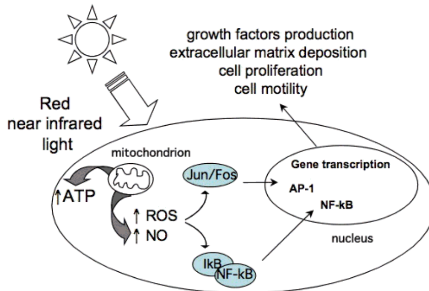
Figure 5. Cell signaling pathways induced by LLLT
